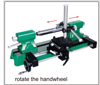
straightness measurement
