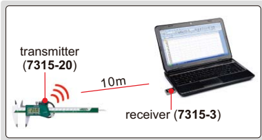
7315-3 application (single channel)
